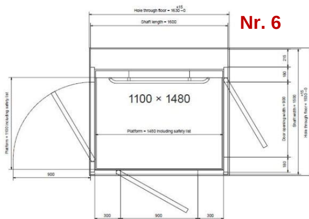
Hul i gulv, L x B = 1630 x 1530 mm. (+15,-0) Skakt, L x B = 1600 x 1500 mm.
