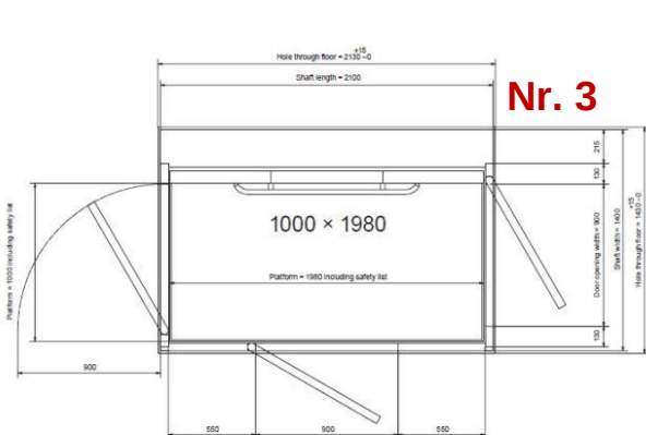
Hul i gulv, L x B = 2130 x 1430 mm. (+15,-0) Skakt, L x B = 2100 x 1400 mm.
