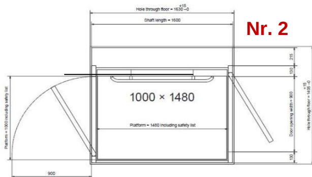
Hul i gulv, L x B = 1630 x 1405 mm. (+15,-0) Skakt, L x B = 1600 x 1375 mm.
