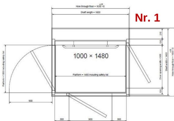
Hul i gulv, L x B = 1630 x 1430 mm. (+15,-0) Skakt, L x B = 1600 x 1400 mm.
