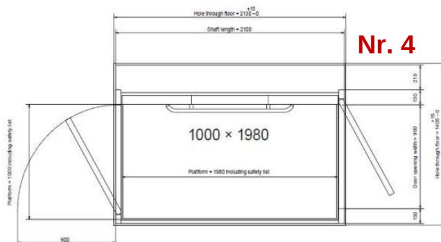
Hul i gulv, L x B = 2130 x 1405 mm. (+15,-0) Skakt, L x B = 2100 x 1375 mm.
